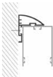
Front Fix standard 40 x 43 mm
